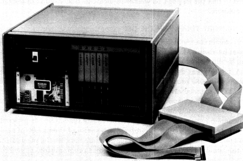
Fig. 5—Hardware development system (DSPMATE).
